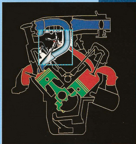
Smooth power is supplied by Grand Marquis' 5.0-liter V-8. The engine features sequential multi-port electronic fuel injection to enhance performance and fuel economy.*
