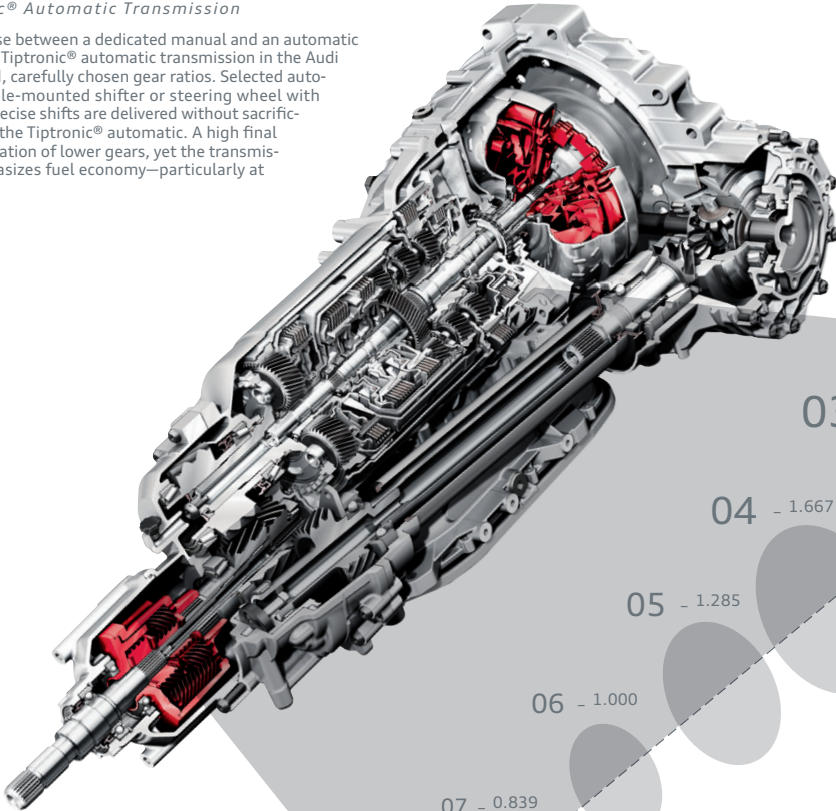
.16 – Eight-speed Tiptronic® Automatic Transmission
