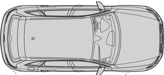
.24 – Audi Side Assist The available Audi side assist uses radar sensors and two different optical warnings to help keep the driver informed of what is approaching from hard-to-see angles behind and to the side of the vehicle.
