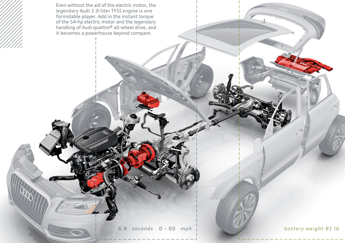
.20 - 2.0 TFSI with quattro®
