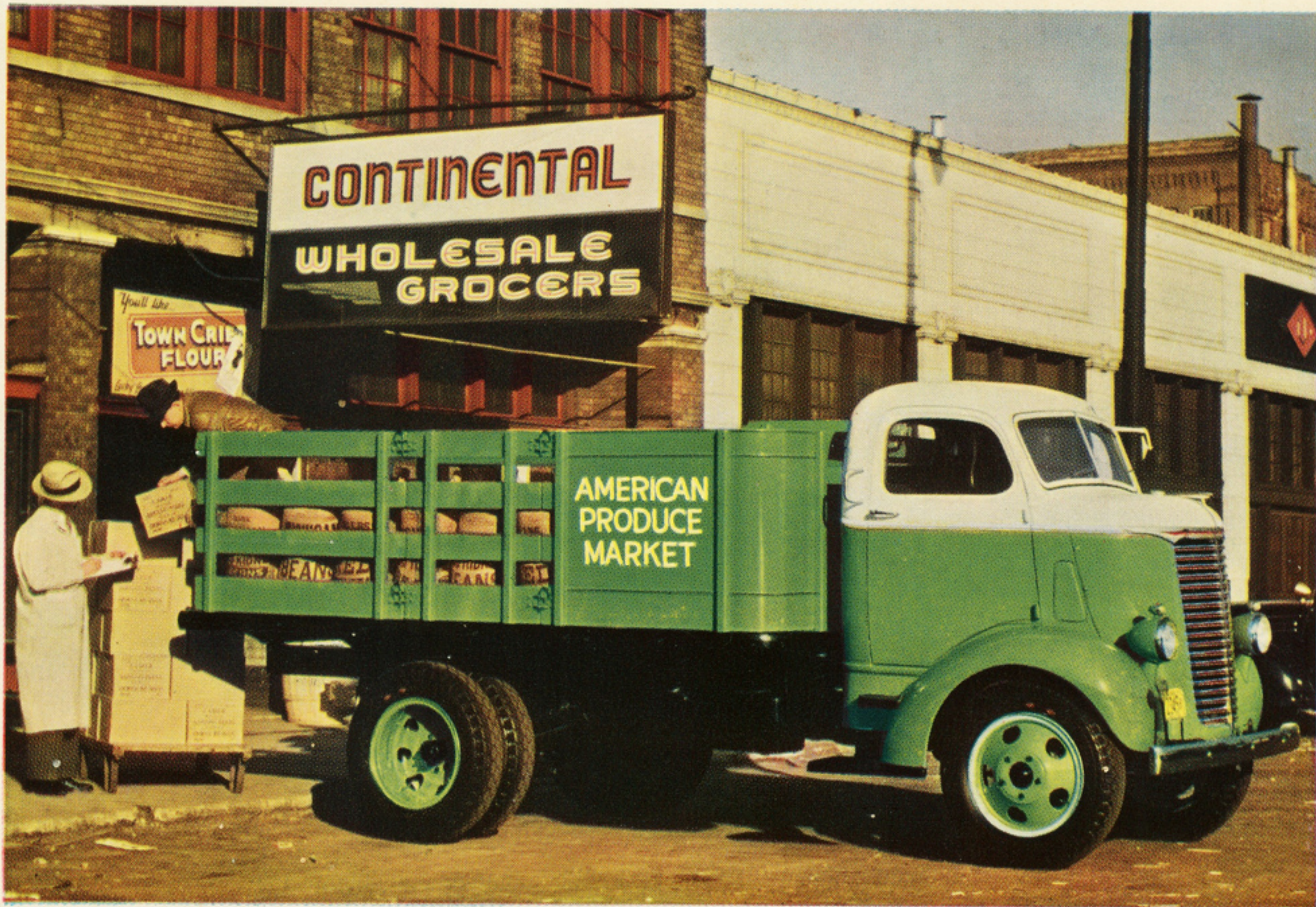
CHEVROLET HEAVY-DUTY CAB-OVER-ENGINE STAKE TRUCK — 1½-Ton Capacity 131½-Inch Wheelbase. Load Space: 141½ inches long, 80¾ inches wide, 38½ inches high
