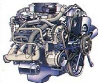
Available 4.3 Liter Vortec V6 (now standard on Safari Passenger Vans) with new electronic fuel injection delivers impressive performance. Develops 145 SAE net horsepower at 4000 RPM. Features new high-output 85-amp generator as standard equipment.
