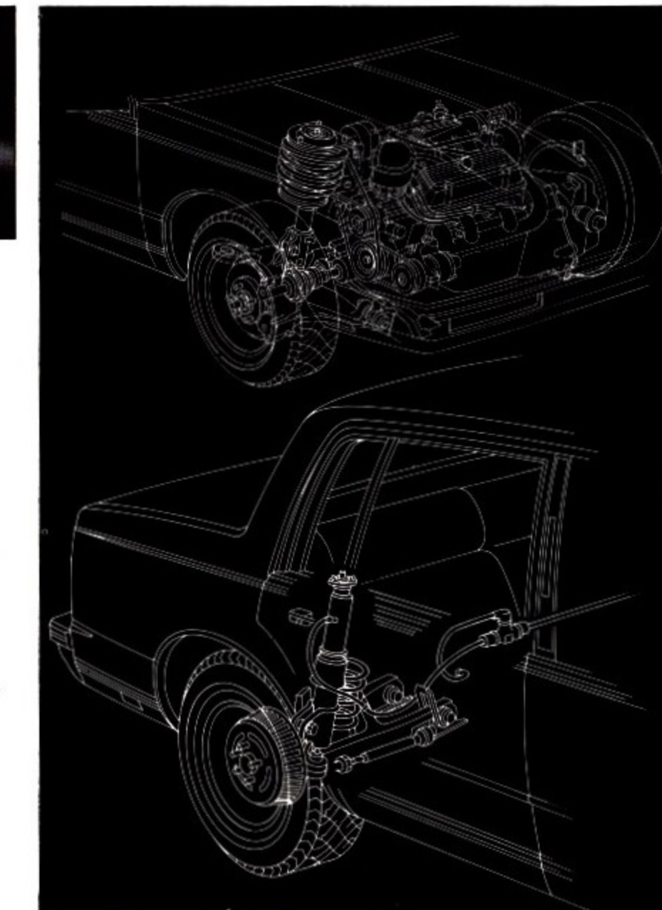
Delta 88 Royale performance team. Front-wheel drive. Four-wheel independent suspension with MacPherson front struts. Power rack-and-pinion steering. Available 3.8 Litre V6 with Sequential-Port Fuel Injection.
