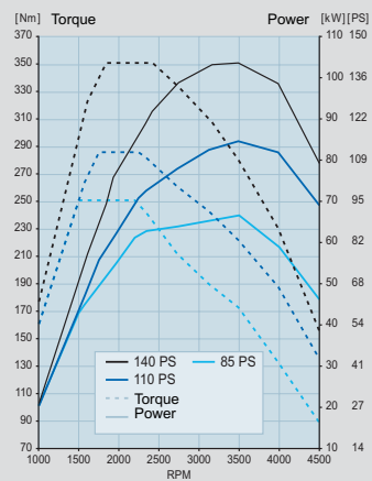
Diesel (FWD)
